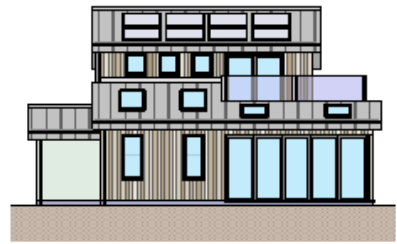
PROPOSED SIDE ELEVATION facing south-west
