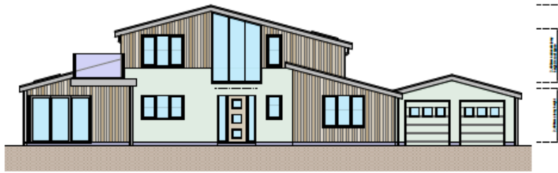
PROPOSED FRONT ELEVATION facing south-west
